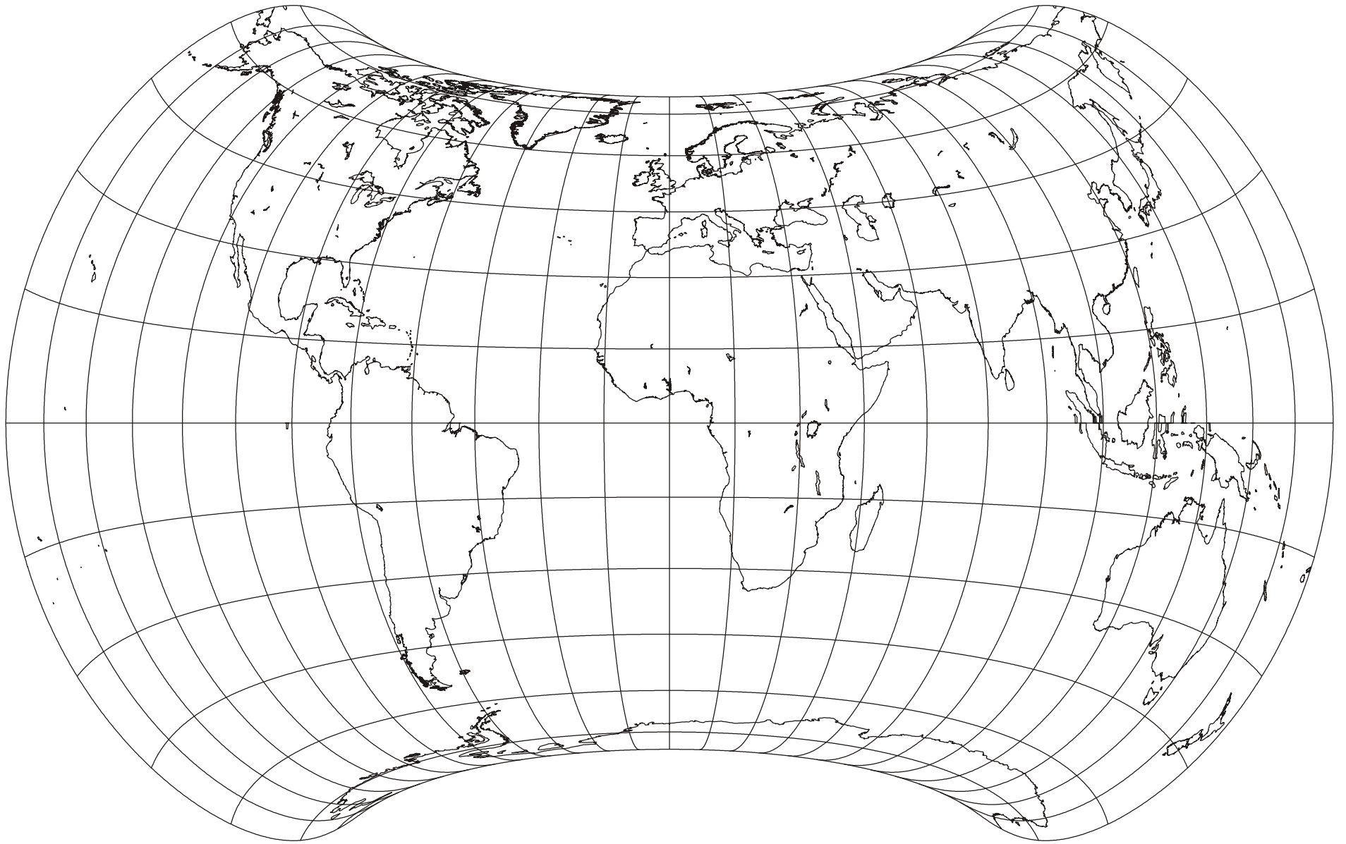
Strebe Equal-area projection; Polyconic; Daan Strebe; 1995
